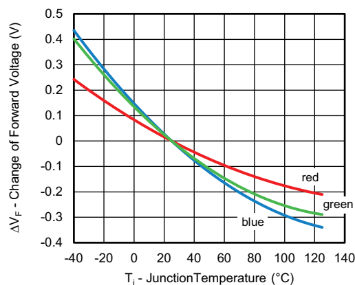
Fig. 14 - Change of Forward Voltage vs. Junction Temperature
