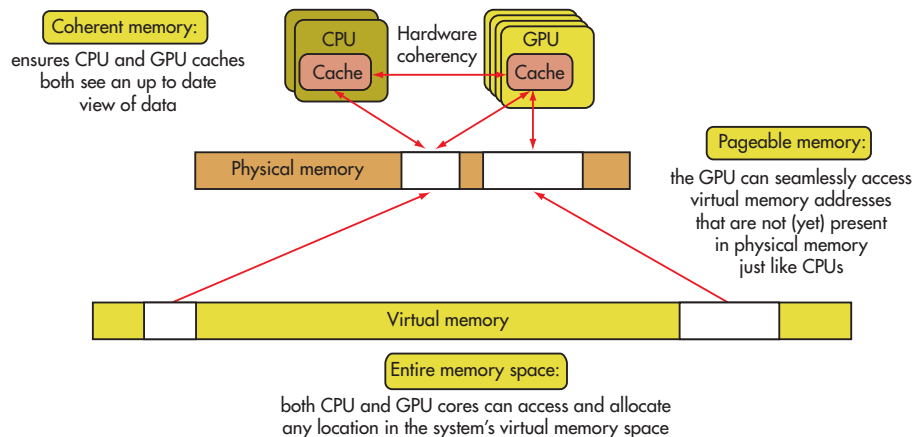
1. AMD's Heterogeneous System Architecture (HSA) allows CPU and GPU cores to use the same virtual memory address space so data does not have to be copied for use by different types of cores. This greatly simplifies programming and considerably improves speed.
