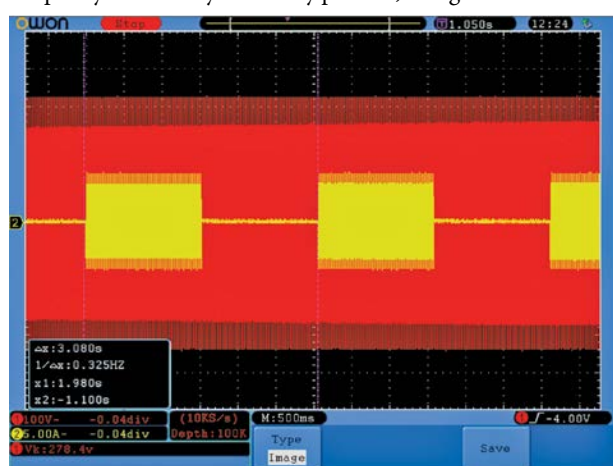
8. This is a load modulation pattern of 0.325 Hz, i.e., one of the calibration points per Table 5 of IEC 61000-4-15 (the flicker measurement standard). The yellow and red traces represent the current and voltage, respectively. The scope is set to 500 ms/div to record data for several seconds.
