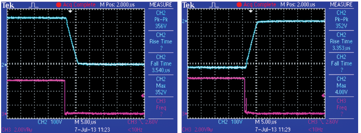
10. The 1- to 5-μs rise/fall times (blue trace) for a 1-cycle drop-out starting and ending at 90°.
