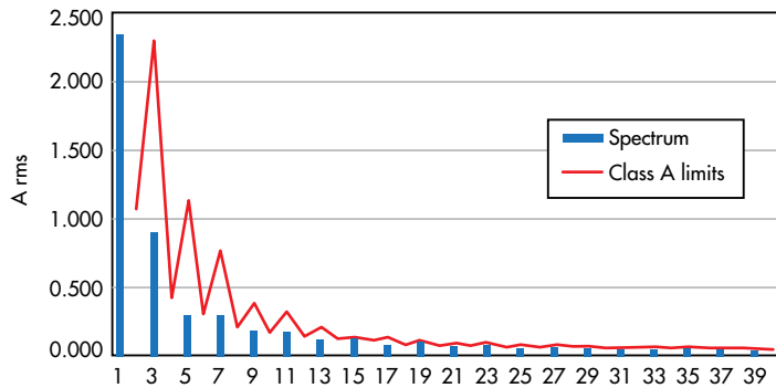
4. Spectrum from H1-H40 for an 80-Ω load when conducting current from 45° to 135°.
