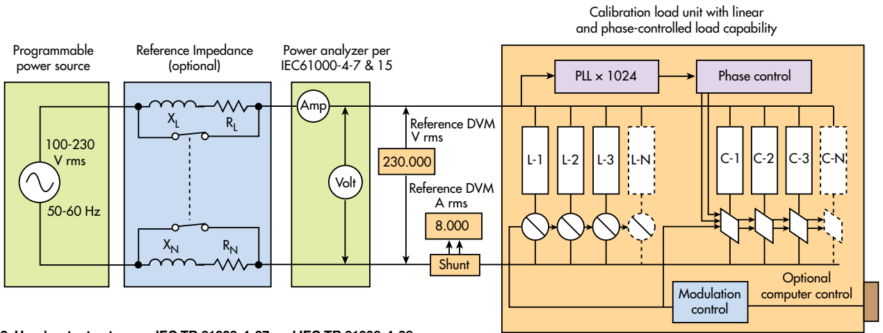
2. Here's a test setup per IEC TR 61000-4-37 and IEC TR 61000-4-38
