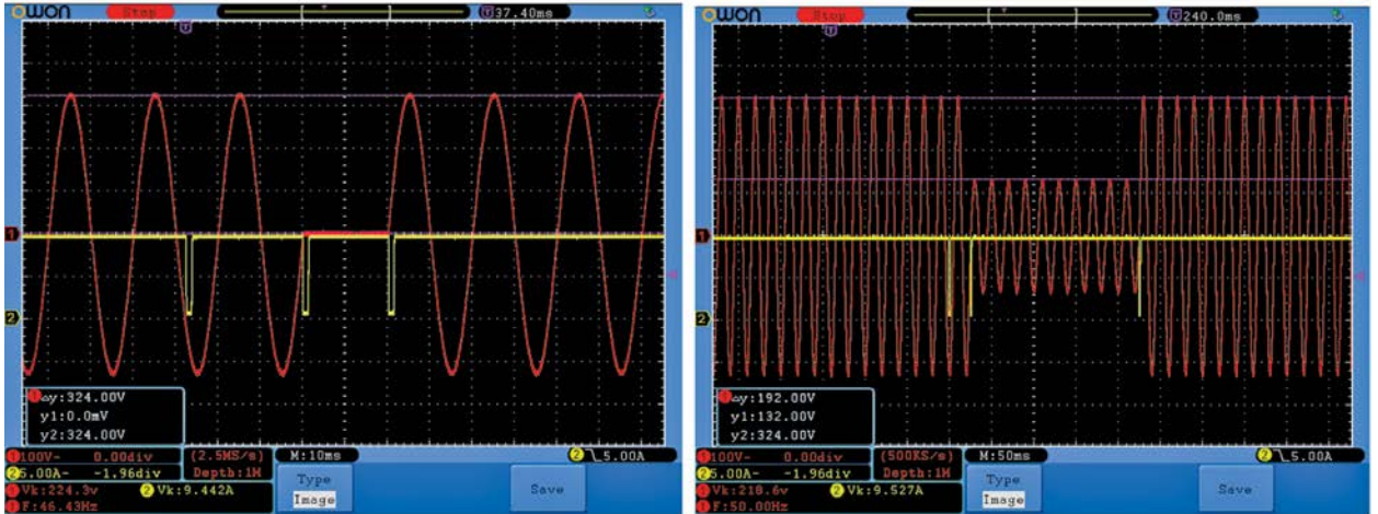
9. Shown are a 1-cycle drop-out to “0” V (left) and a dip to 40 % remaining for 10 cycles (right)
