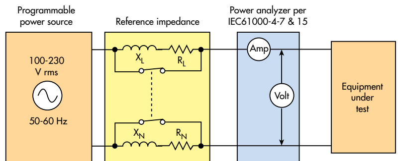
1. This harmonics and flicker test system, which is a typical setup, is shown with the impedance in bypass mode for harmonics testing.
