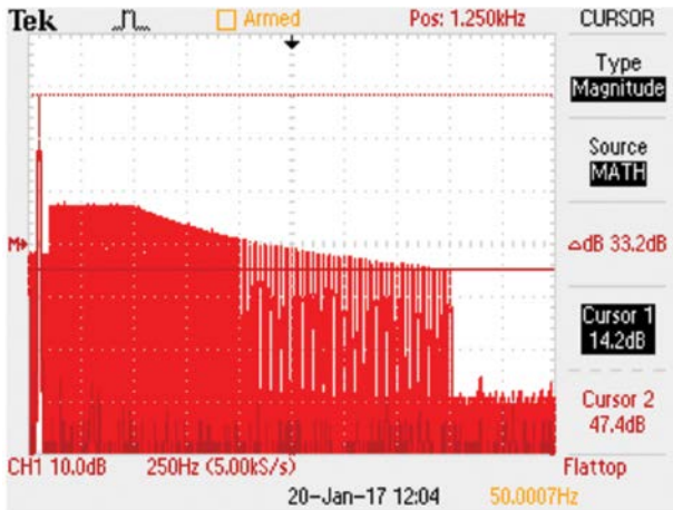
11. Meister curve sweep test from 16 Hz to 2000 Hz per Class-2.
