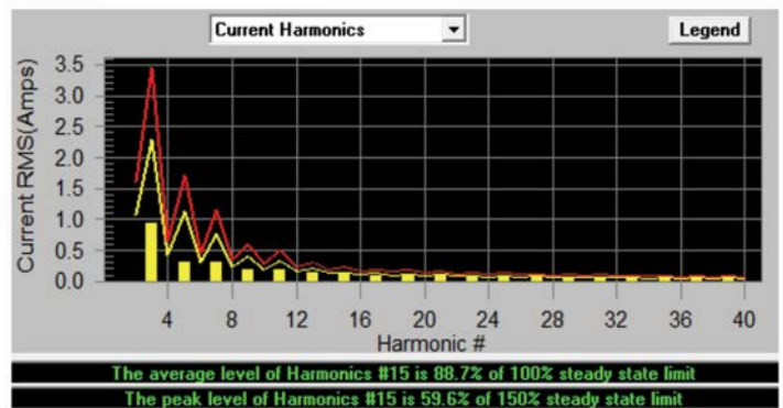
3. Waveform and current spectrum passing IEC 61000-3-2 Class-A with 88.7% of the limits (blue trace is current on the left; yellow bars on the right are harmonics along with the 100% yellow limit line and 150% red limit line).
