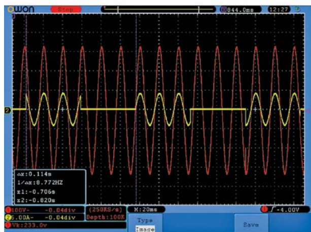
7. Depicted is the 8.77-Hz modulation pattern to verify flicker test systems
