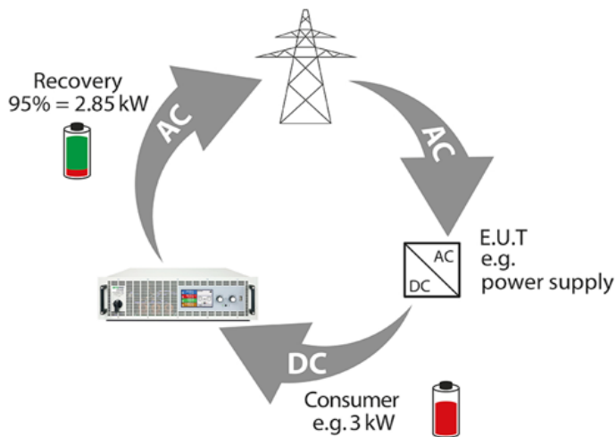
Figure 5: Energy recycling
