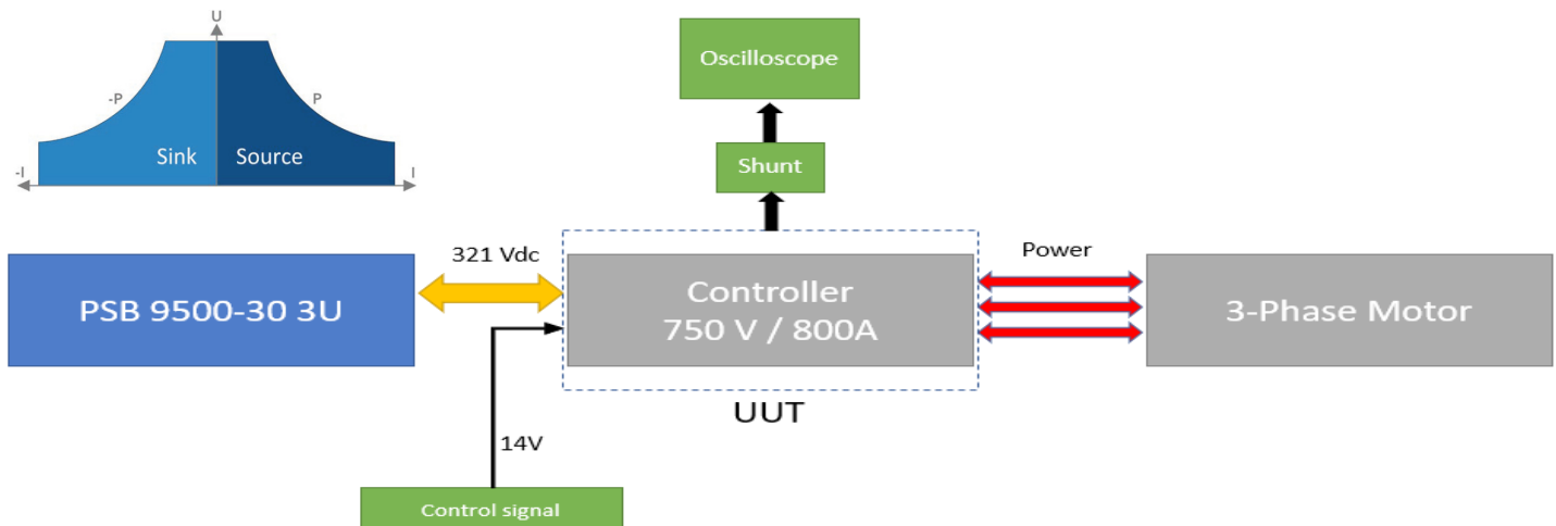
Figure 1: Test Setup
