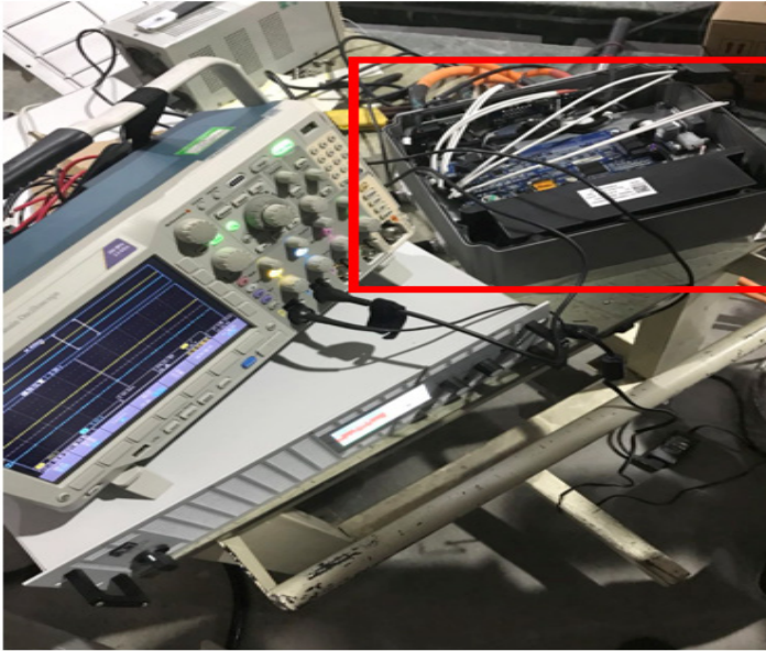
Picture 2: Controller
