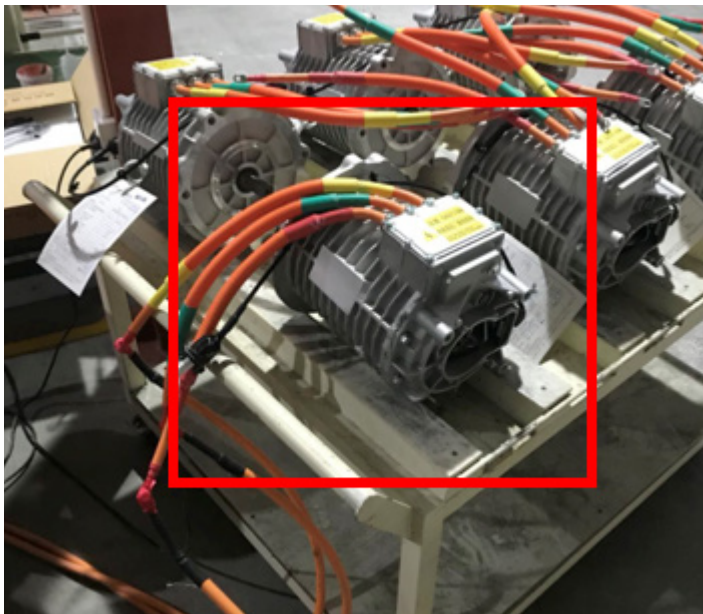
Picture 3: 3-Phase AC Motor
