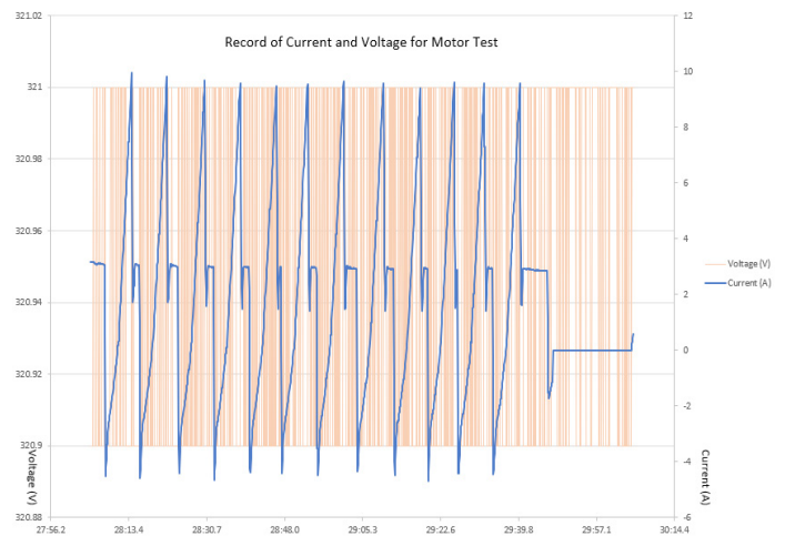
Figure 2: Voltage and current trace, 100msec sample rate.
